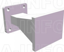
LB-75-10-ASPO Standard Gain Horn Antenna 10-15GHz 10dB Gain Rectangular Waveguide Interface
