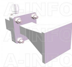
LB-75-10-C-TFSPO Standard Gain Horn Antenna 10-15GHz 10dB Gain TNC Female
